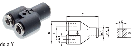
Raccordo a Y
